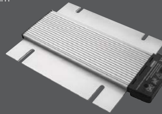
Electric Heater 230V, 380Watts Size 198×297mm
